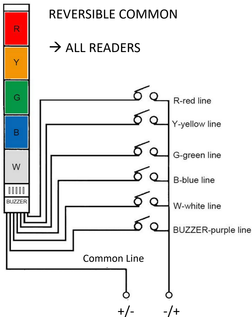
Figure 10 A REVERSIBLE COMMON configuration. This can work with all SensThys readers.
